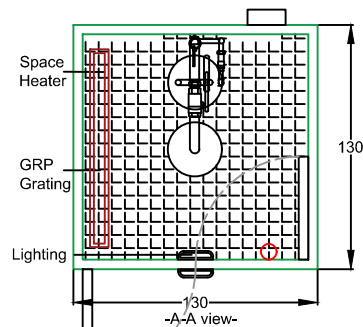
-A-A view-
